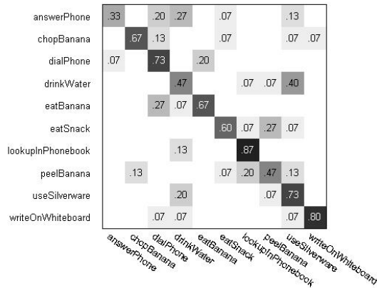
Figure 2. Confusion matrix using only feature trajectory information without augmentations. Overall accuracy is 63%. Zeros are omitted for clarity
